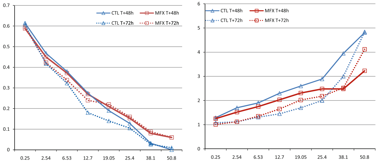
Fig. 7 Equitable Threat Score ( left ) and Bias Score ( right ) of Eta model forecasts of precipitation using the original Kain-Fritsch (triangles) and included momentum transports (squares) schemes,
