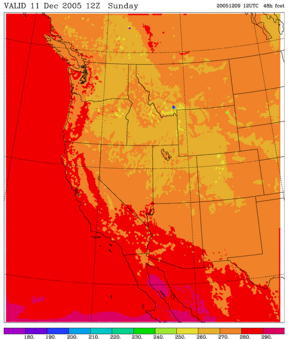
Fig. 4 Lowest layer temperatures obtained when using scheme (2) for the slantwise temperature advection, in a 48-h forecast verifying at 1200 UTC 11 December 2005
