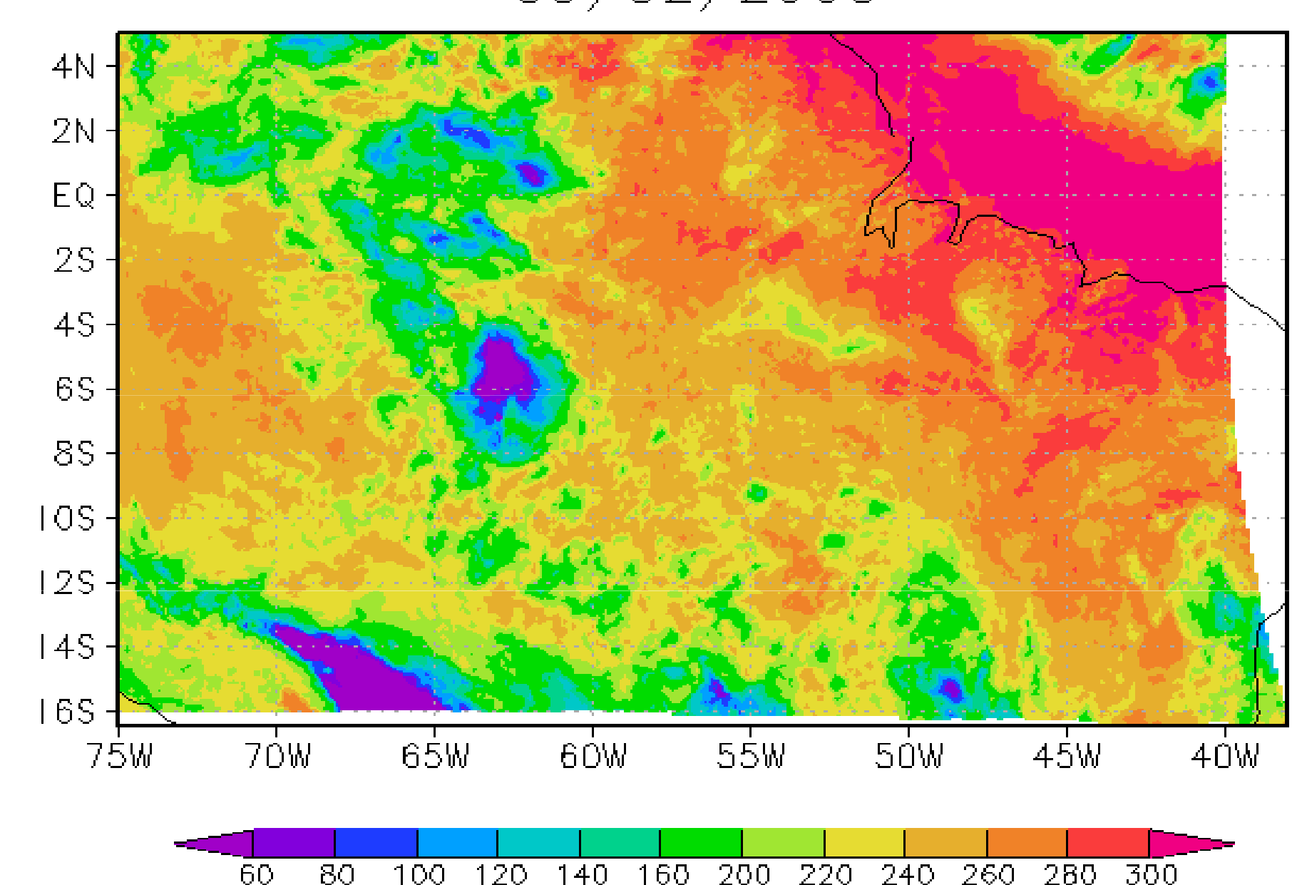
Figure C Daily SW surface downward flux at 1/8 deg. 09/02/2000
