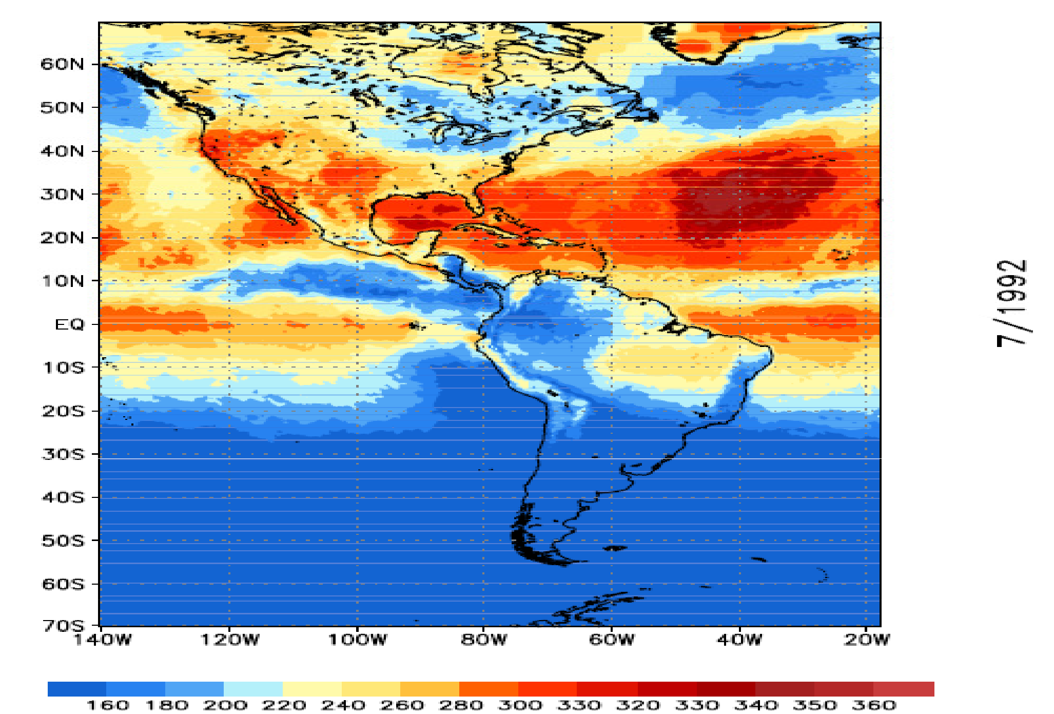
Figure B Monthly mean shortwave surface downwelling flux (w/m**2) gridded to 0.5 Deg merged from ISCCP DX GOES/METEOSAT/AVHRR data
